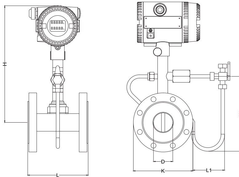
Dimension for Flanged Multi-Variable Type (ANSI CL150)
