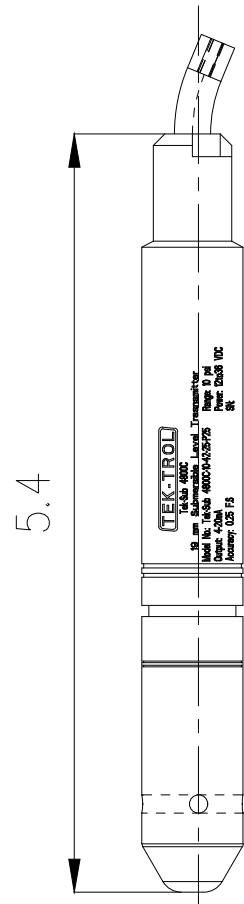
FRONT VIEW
