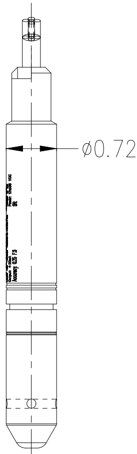
RH VIEW
